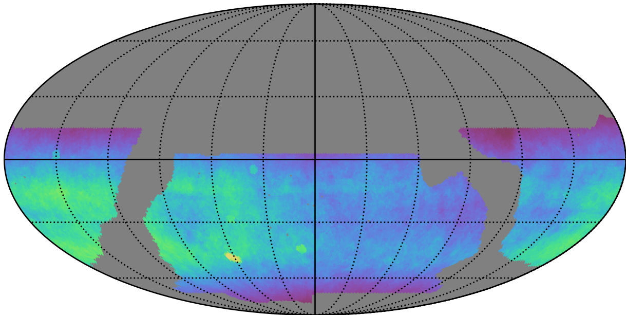
baseline_v2.1_10yrs WFD i band: Normalized Teff
