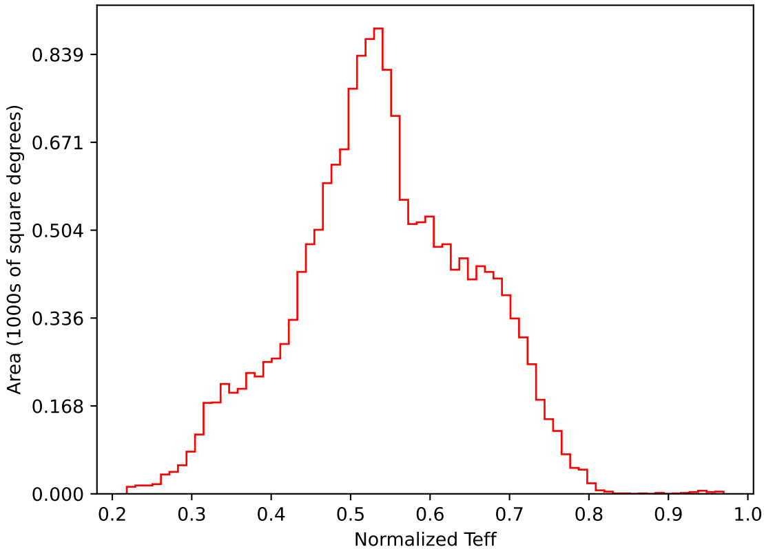
baseline_v2.1_10yrs WFD i band: Normalized Teff
