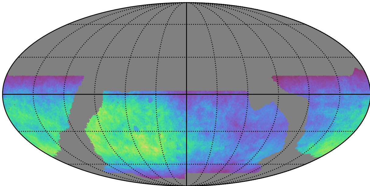
baseline_v2.1_10yrs WFD g band: Normalized Teff
