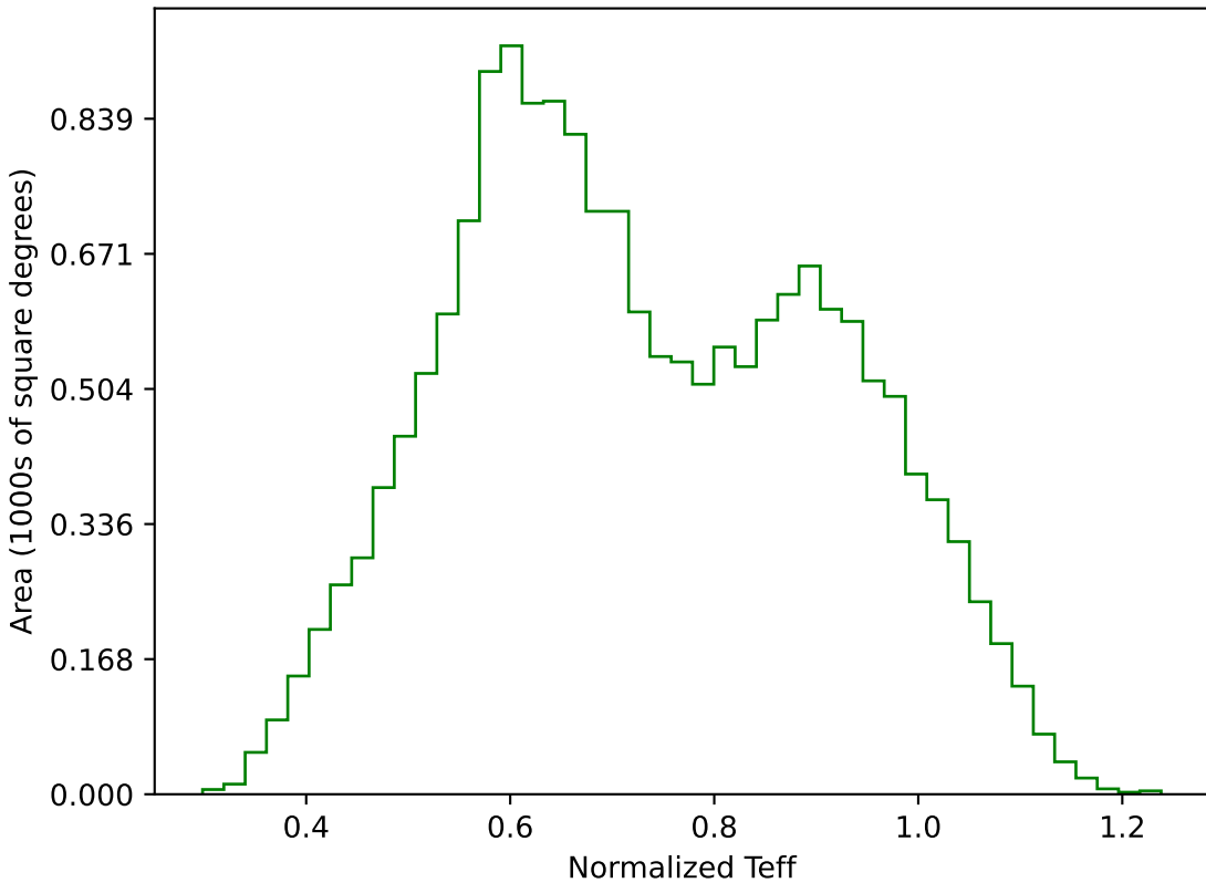
baseline_v2.1_10yrs WFD g band: Normalized Teff
