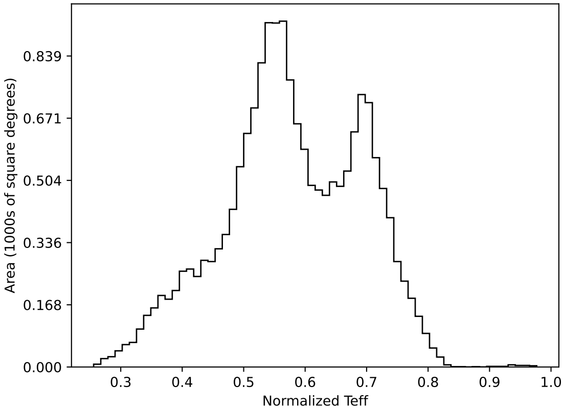
baseline_v2.1_10yrs WFD all bands: Normalized Teff
