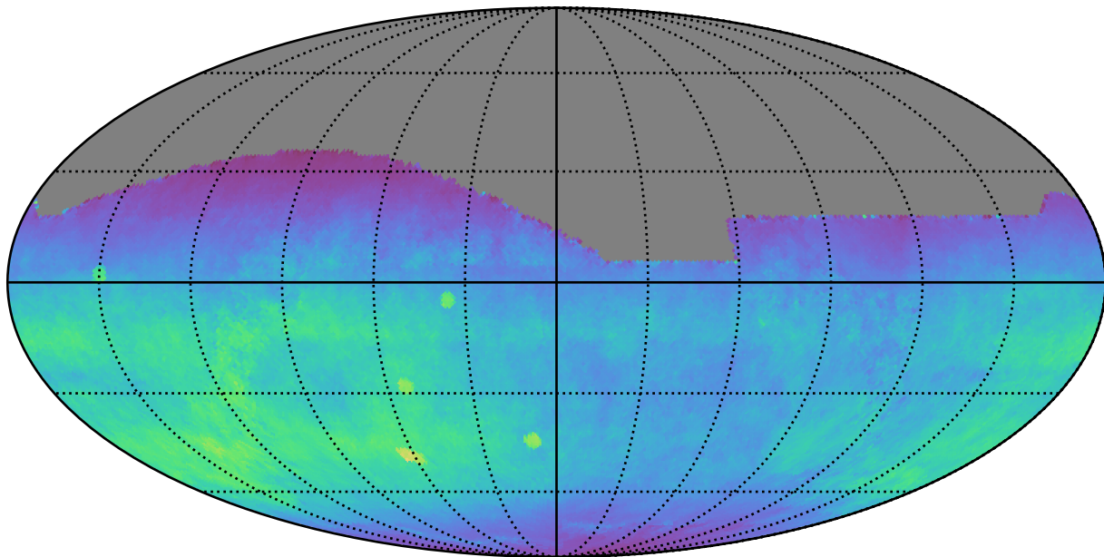
baseline_v2.1_10yrs All sky z band: Normalized Teff
