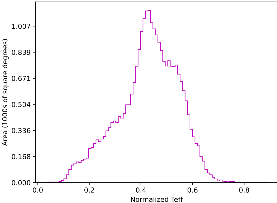
baseline_v2.1_10yrs All sky z band: Normalized Teff
