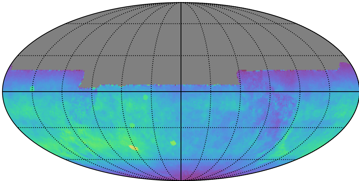
baseline_v2.1_10yrs All sky y band: Normalized Teff
