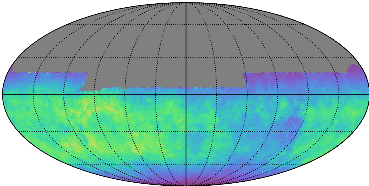
baseline_v2.1_10yrs All sky u band: Normalized Teff
