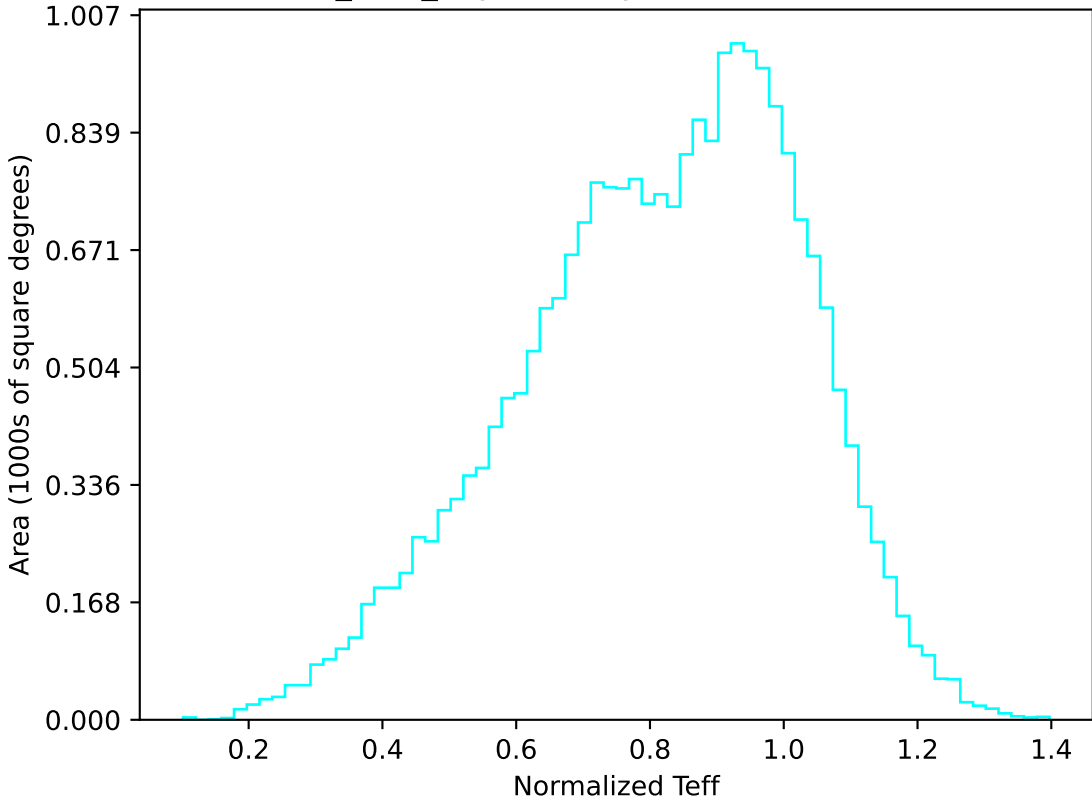
baseline_v2.1_10yrs All sky u band: Normalized Teff
