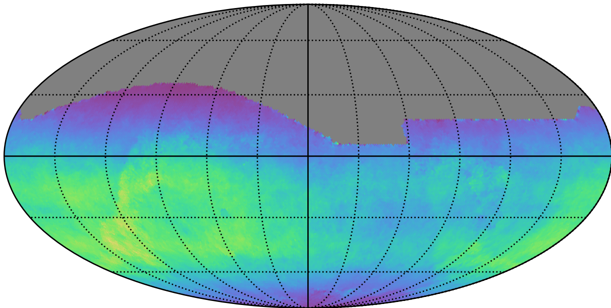
baseline_v2.1_10yrs All sky r band: Normalized Teff
