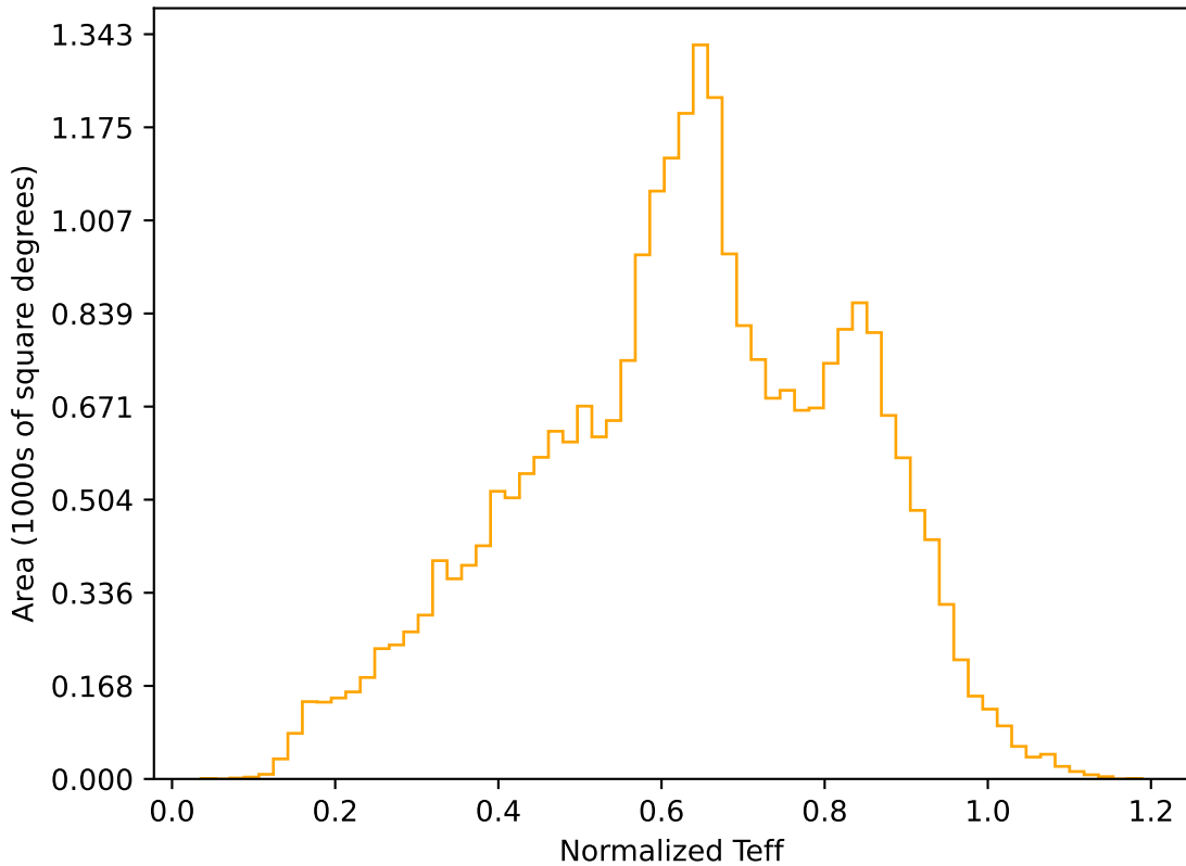
baseline_v2.1_10yrs All sky r band: Normalized Teff
