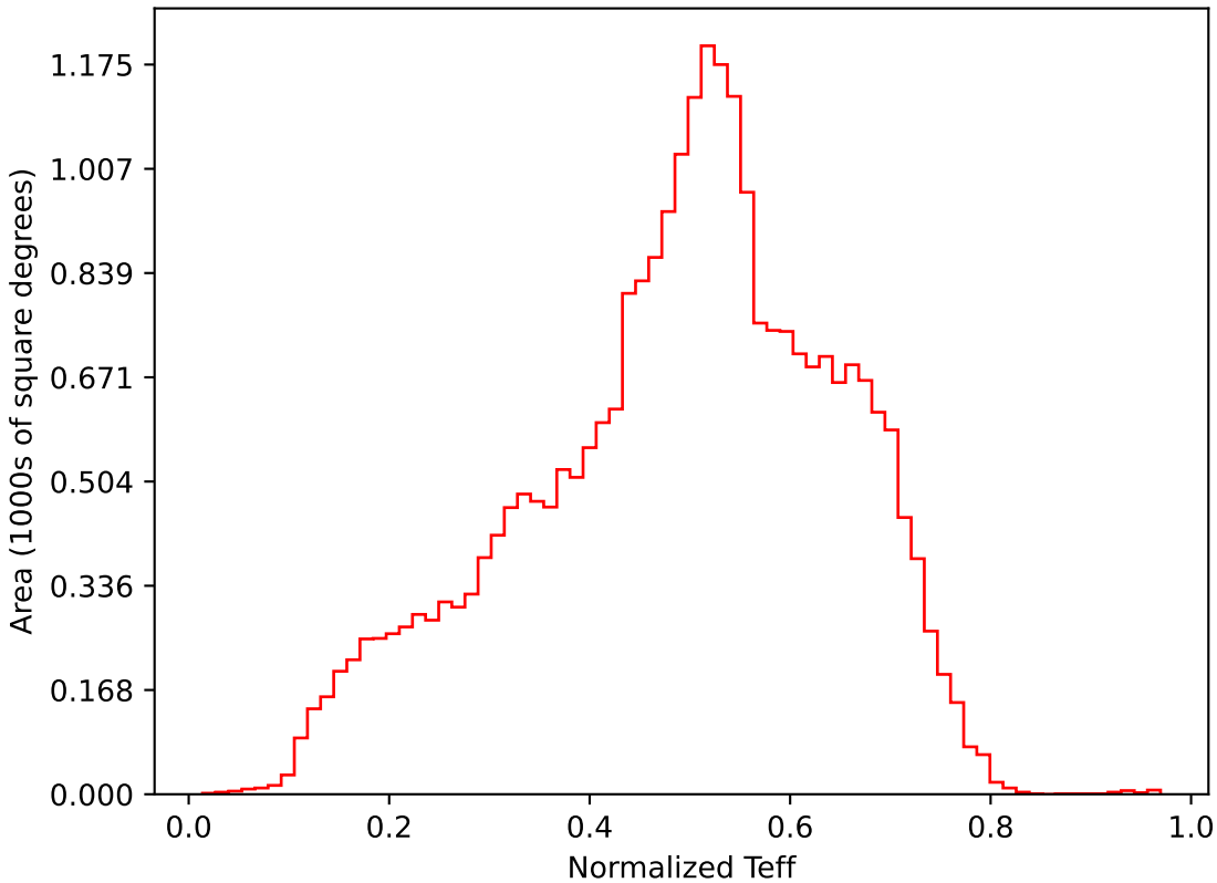
baseline_v2.1_10yrs All sky i band: Normalized Teff
