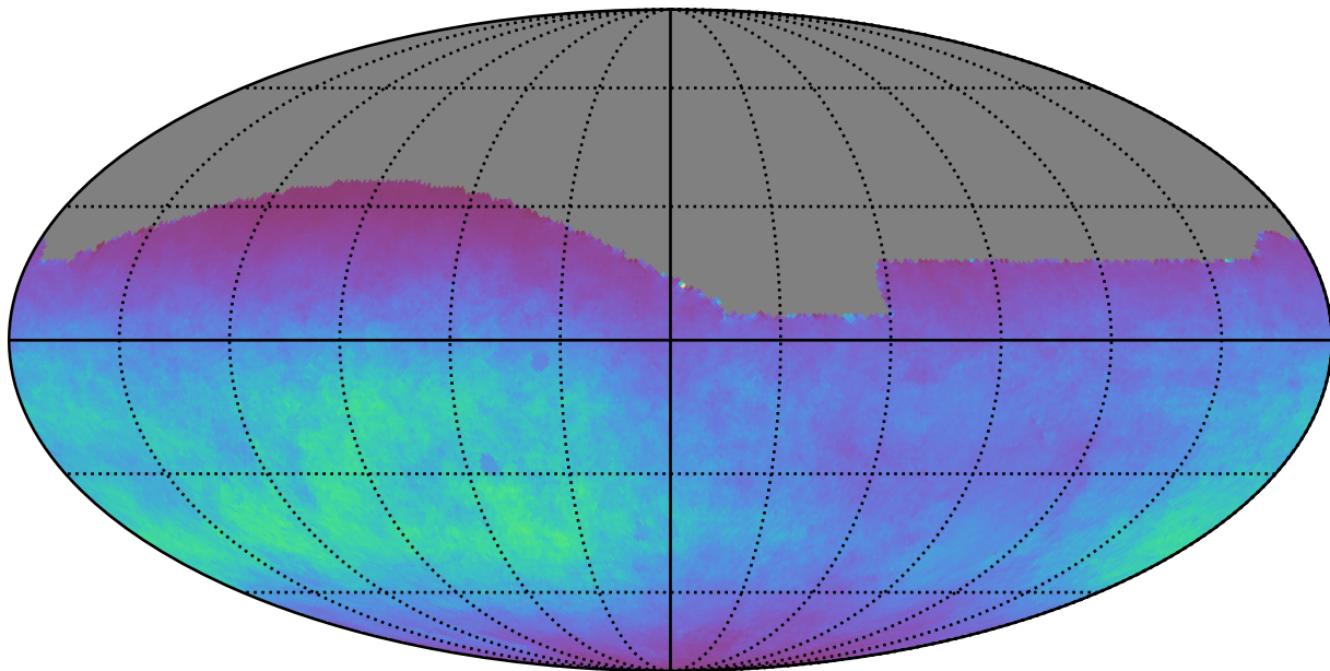
baseline_v2.1_10yrs All sky g band: Normalized Teff
