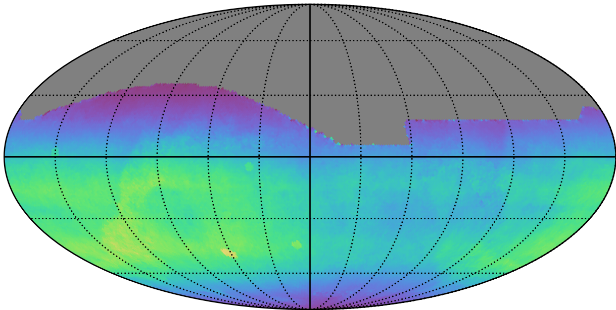
baseline_v2.1_10yrs All sky all bands: Normalized Teff
