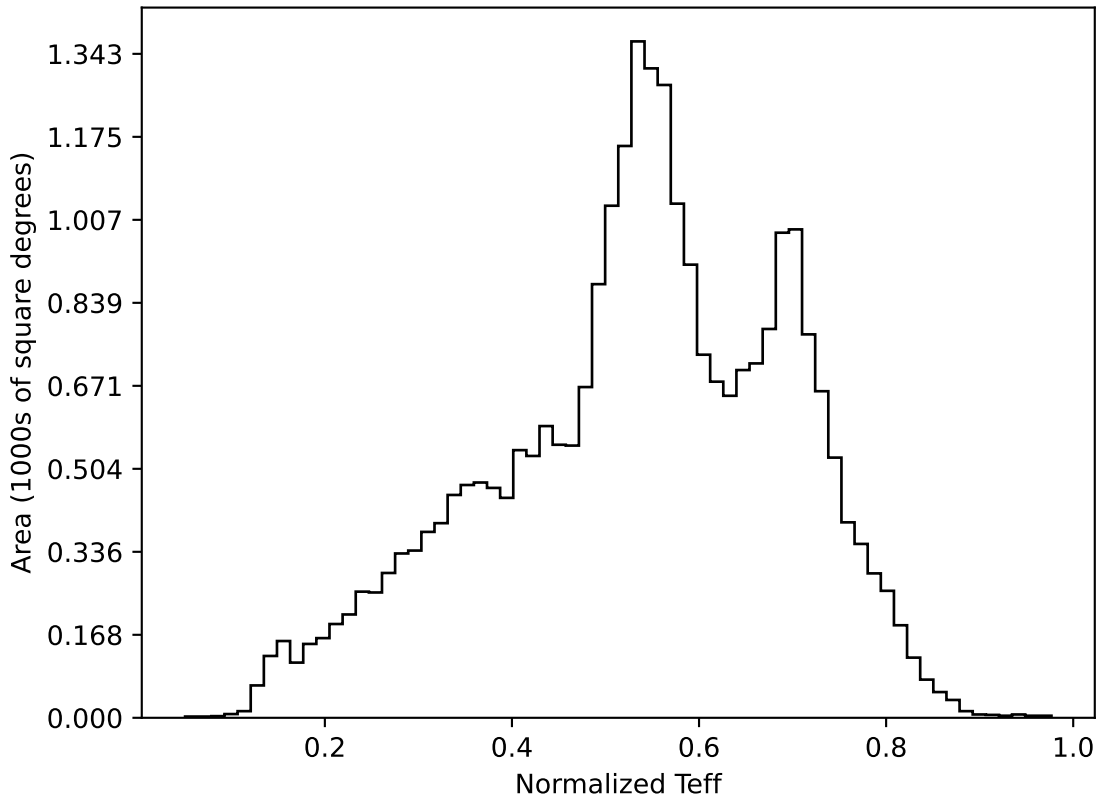
baseline_v2.1_10yrs All sky all bands: Normalized Teff
