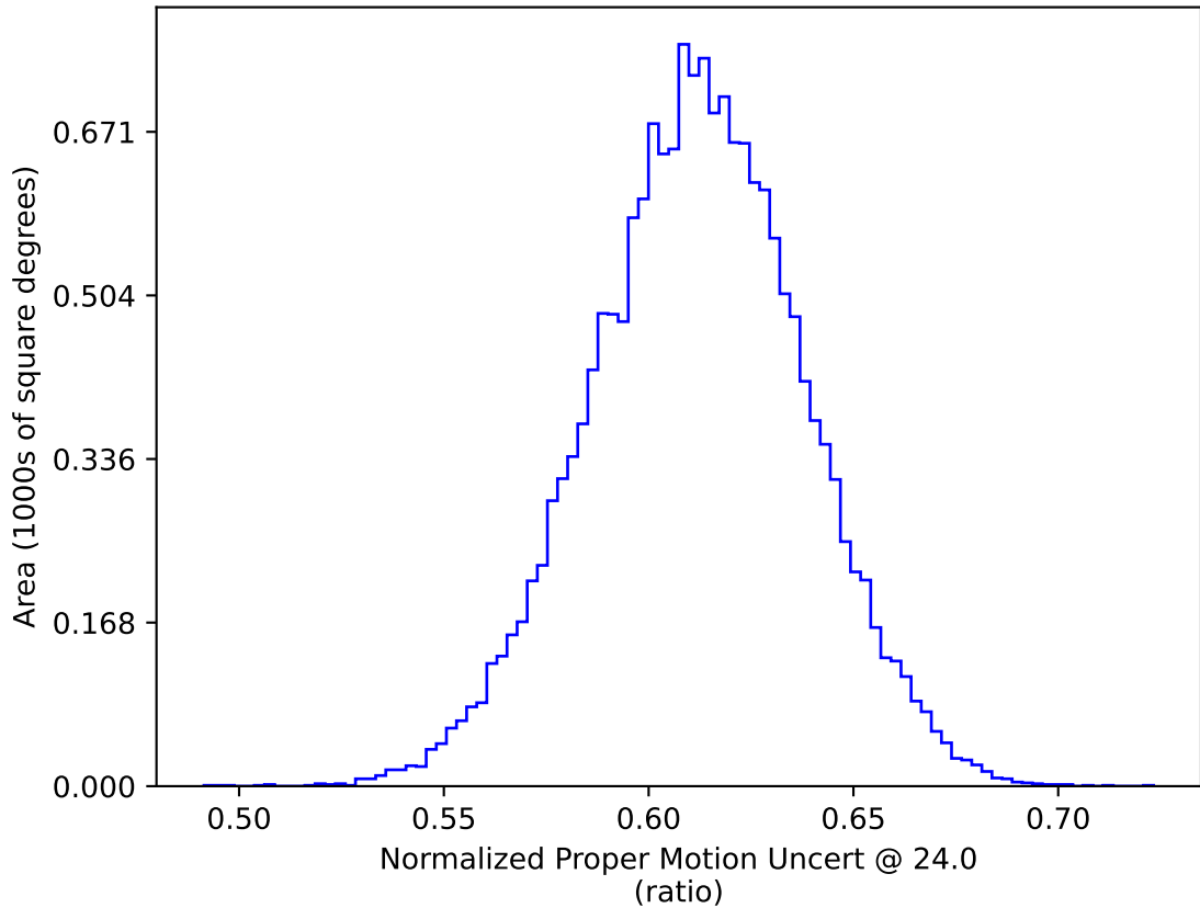
baseline_v2.1_10yrs WFD: Normalized Proper Motion Uncert @ 24.0
