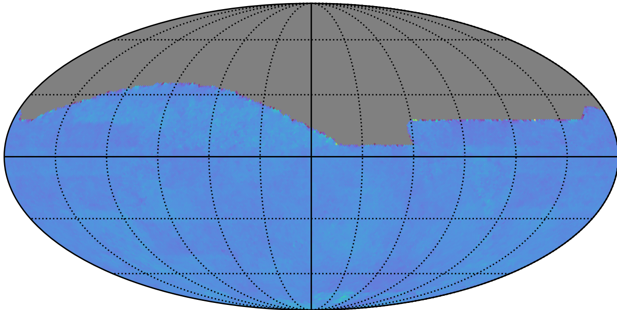
baseline_v2.1_10yrs All sky: Normalized Proper Motion Uncert @ 24.0
