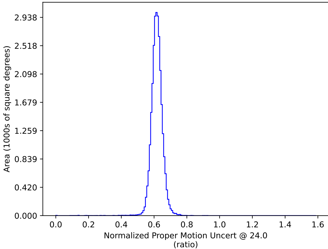
baseline_v2.1_10yrs All sky: Normalized Proper Motion Uncert @ 24.0
