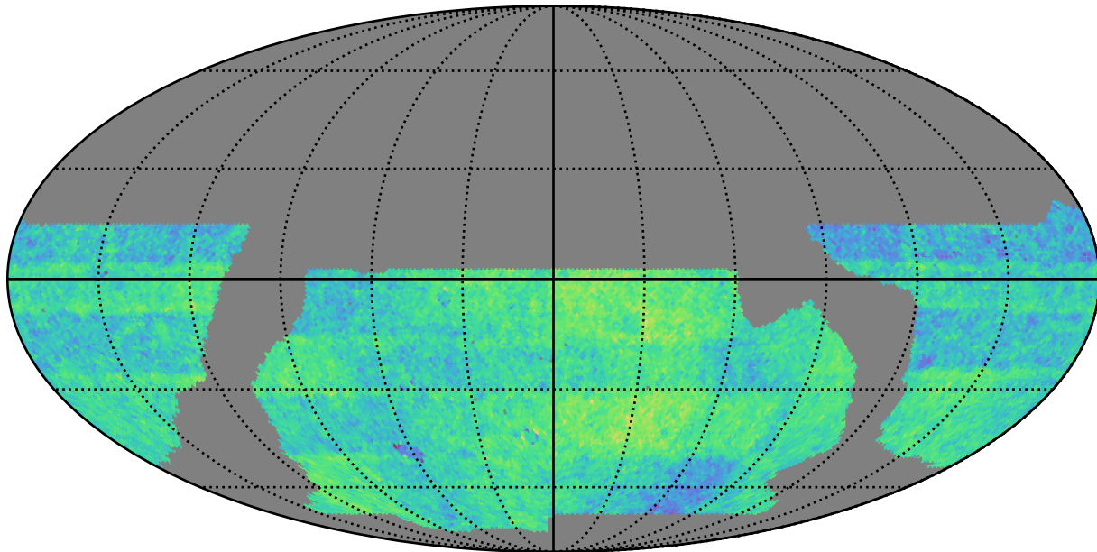
baseline_v2.1_10yrs WFD: Normalized Proper Motion Uncert @ 20.5
