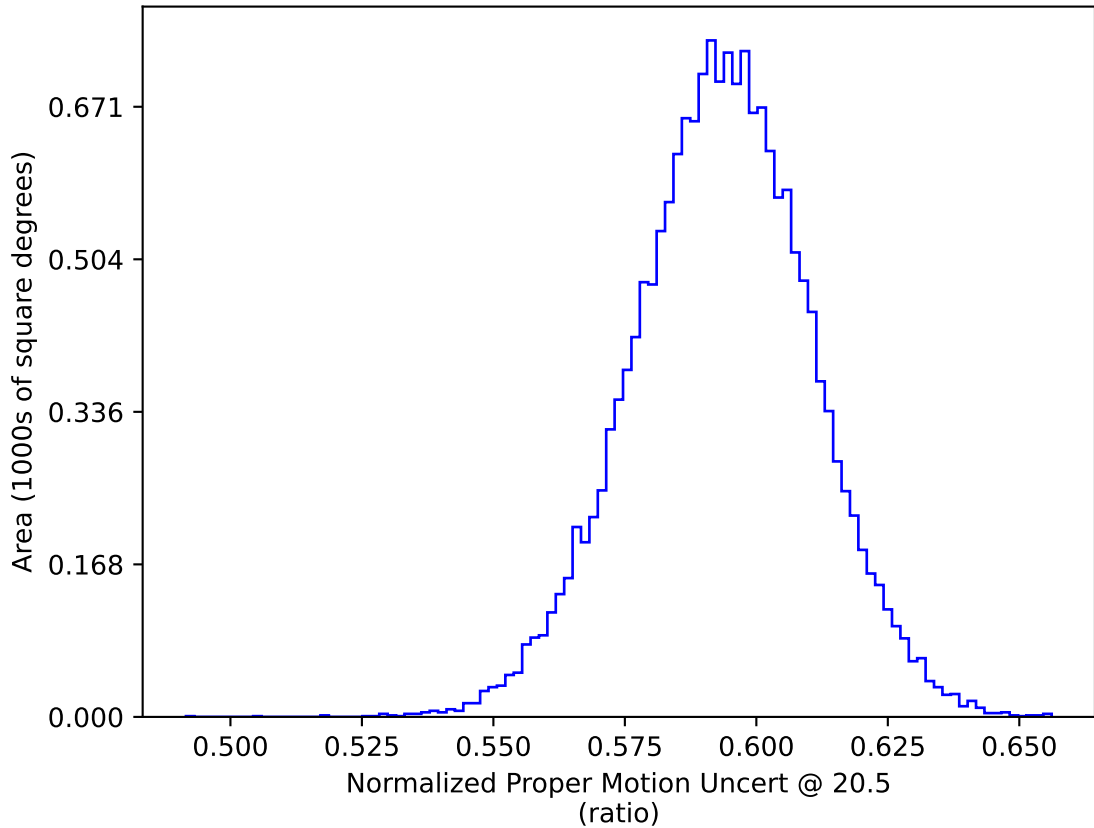
baseline_v2.1_10yrs WFD: Normalized Proper Motion Uncert @ 20.5
