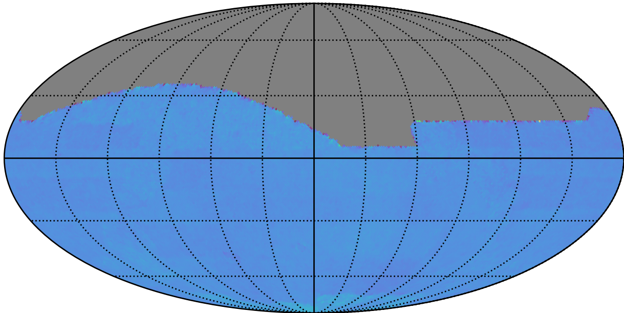
baseline_v2.1_10yrs All sky: Normalized Proper Motion Uncert @ 20.5
