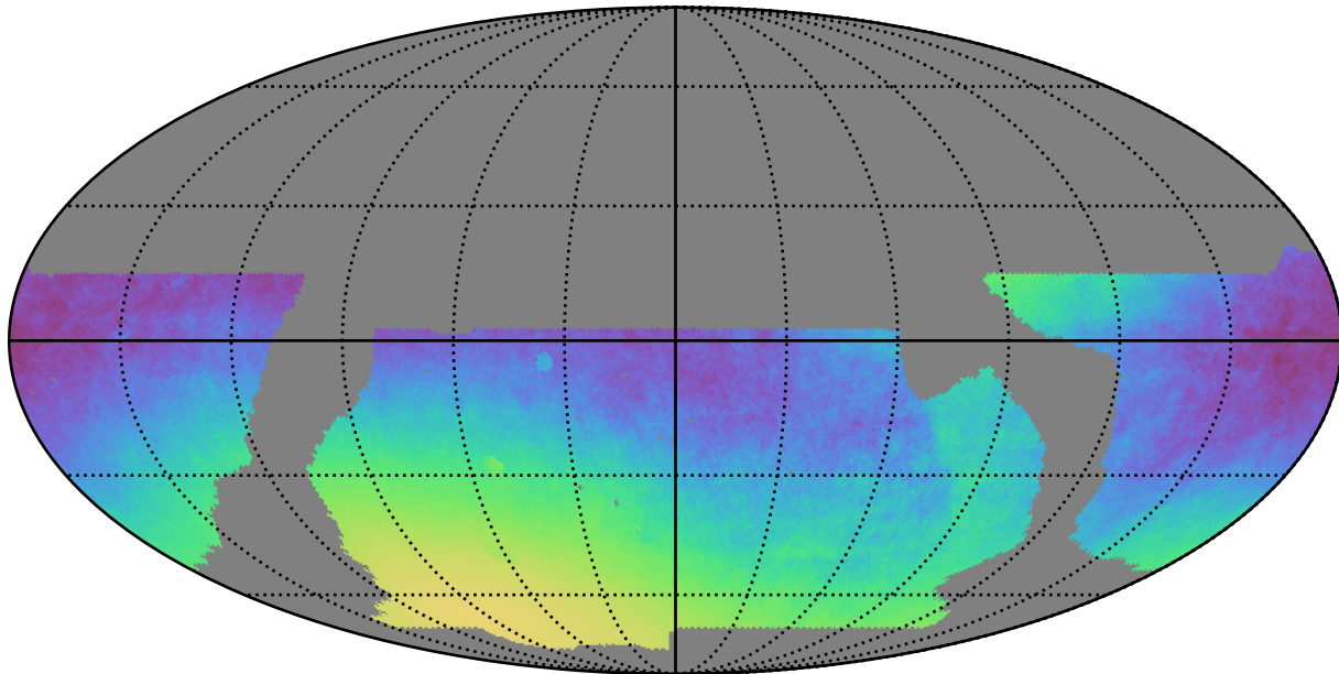
baseline_v2.1_10yrs WFD: Normalized Parallax Uncert @ 24.0
