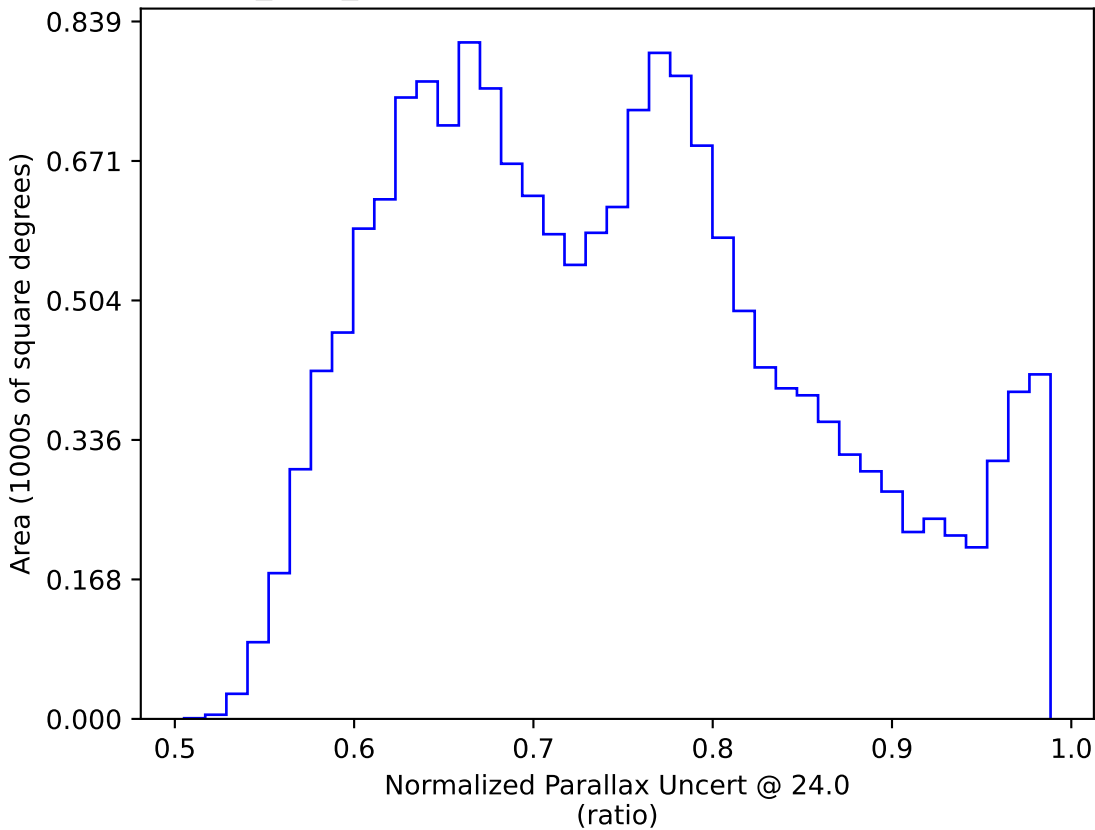
baseline_v2.1_10yrs WFD: Normalized Parallax Uncert @ 24.0
