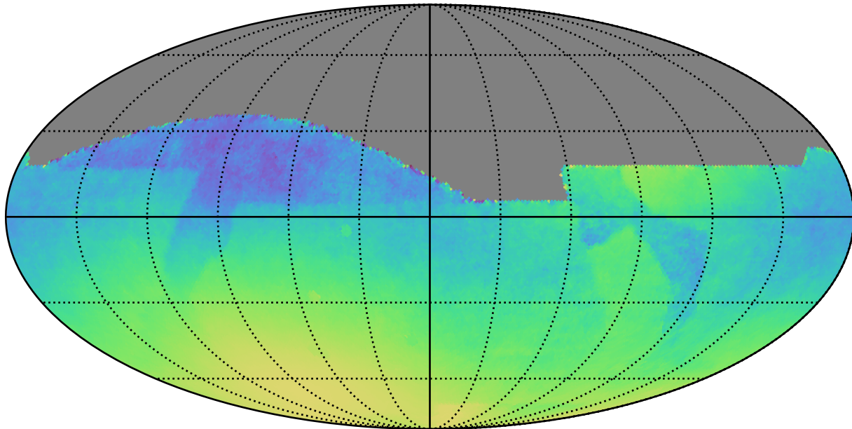
baseline_v2.1_10yrs All sky: Normalized Parallax Uncert @ 24.0
