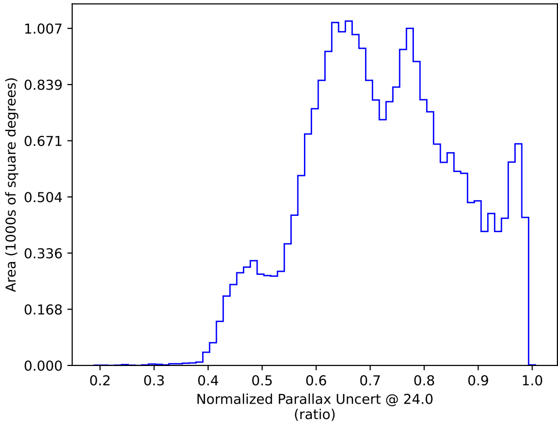
baseline_v2.1_10yrs All sky: Normalized Parallax Uncert @ 24.0
