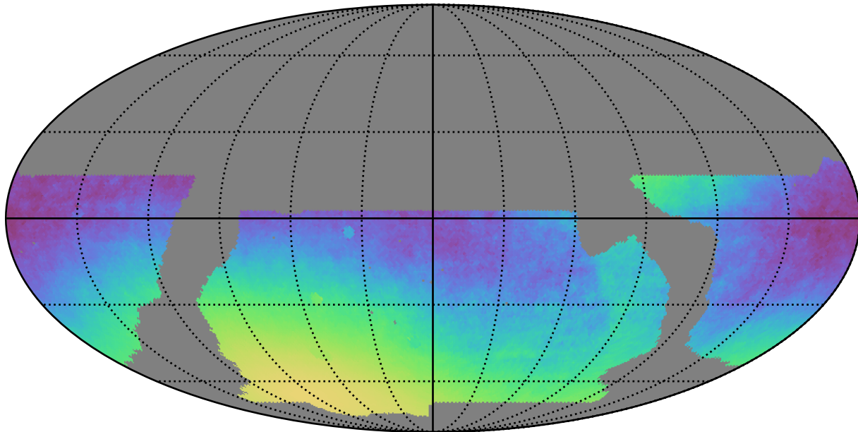
baseline_v2.1_10yrs WFD: Normalized Parallax Uncert @ 22.4
