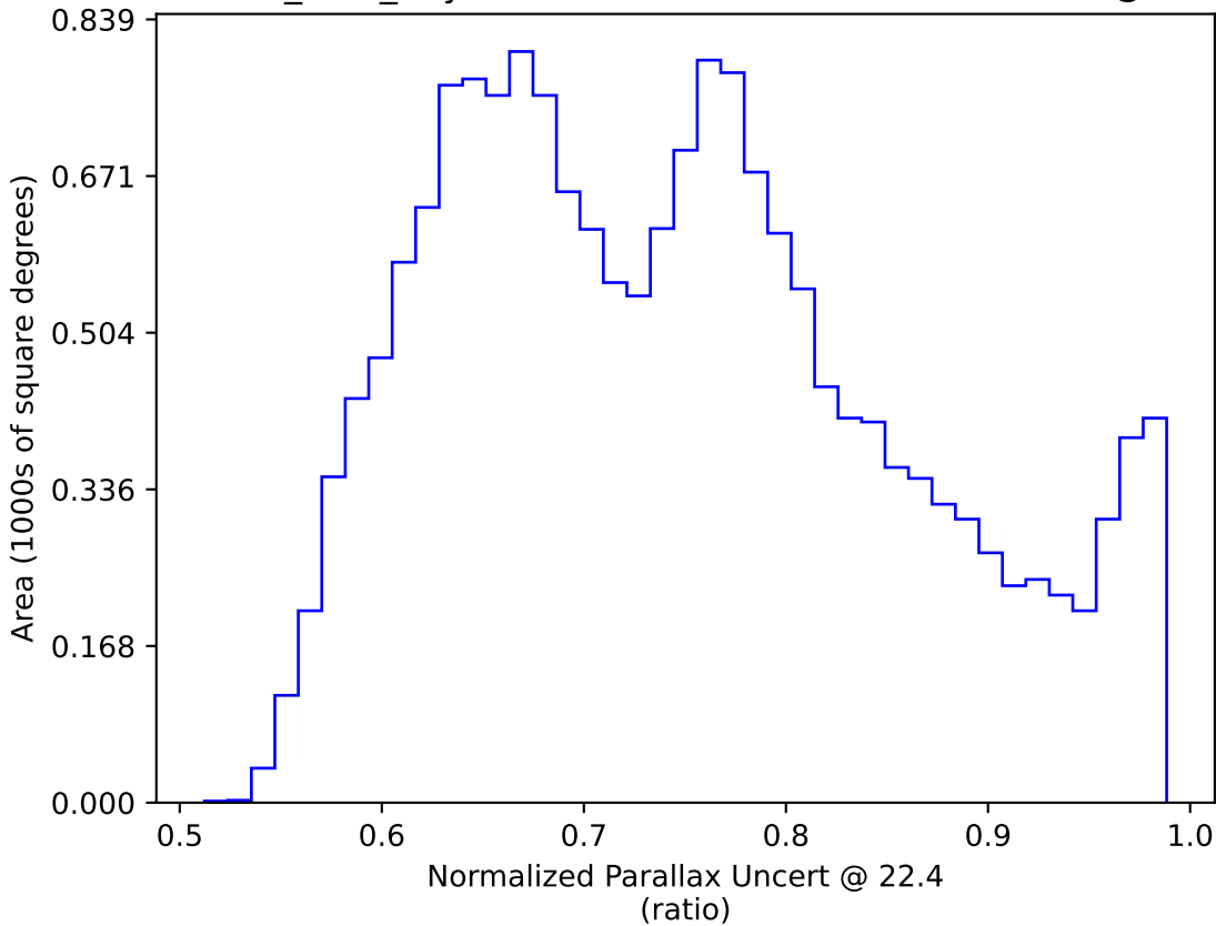
baseline_v2.1_10yrs WFD: Normalized Parallax Uncert @ 22.4
