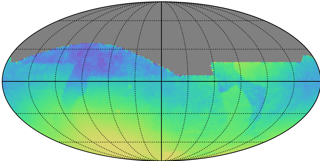
baseline_v2.1_10yrs All sky: Normalized Parallax Uncert @ 22.4
