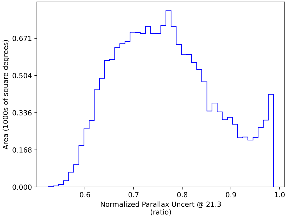
baseline_v2.1_10yrs WFD y band only: Normalized Parallax Uncert @ 21.3
