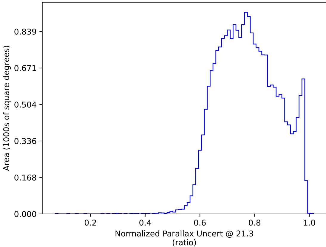
baseline_v2.1_10yrs All sky y band only: Normalized Parallax Uncert @ 21.3
