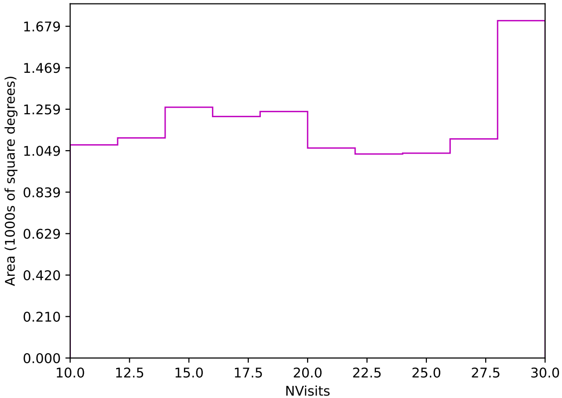
baseline_v2.1_10yrs Yr 3-4 z band: NVisits
