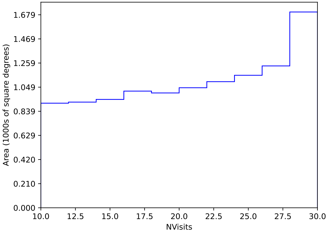
baseline_v2.1_10yrs Yr 3-4 y band: NVisits
