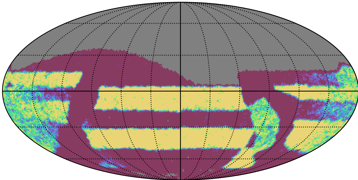
baseline_v2.1_10yrs Yr 3-4 r band: NVisits
