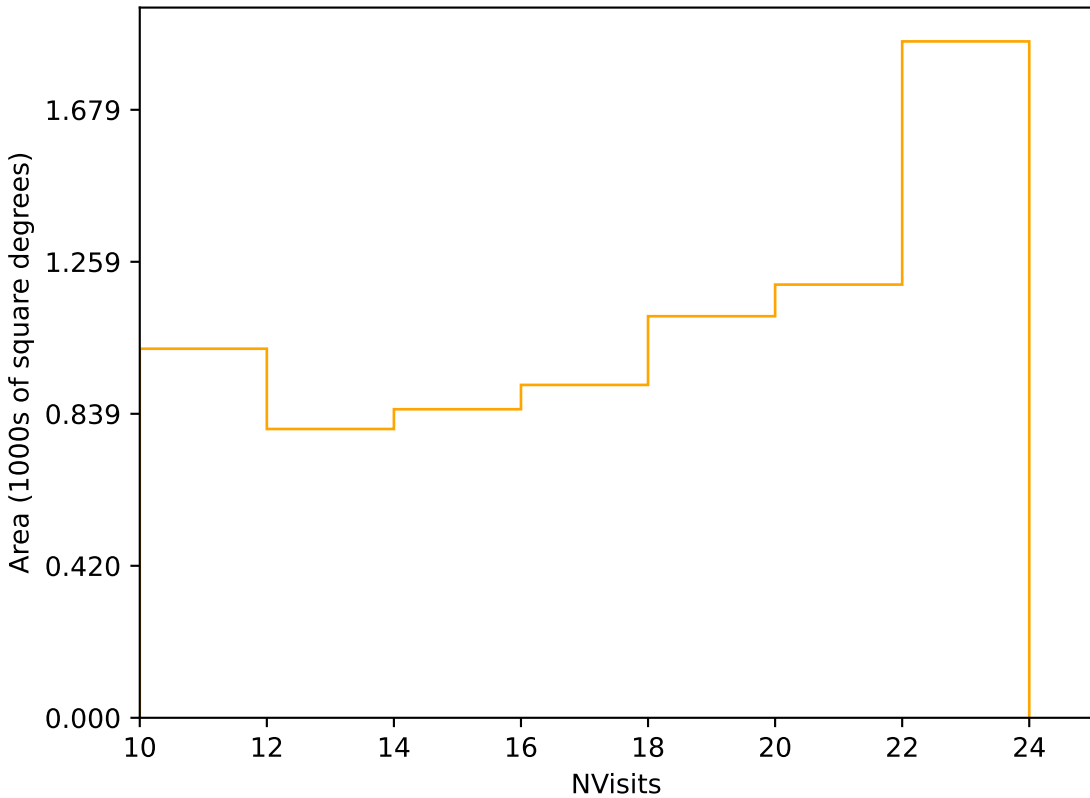
baseline_v2.1_10yrs Yr 3-4 r band: NVisits
