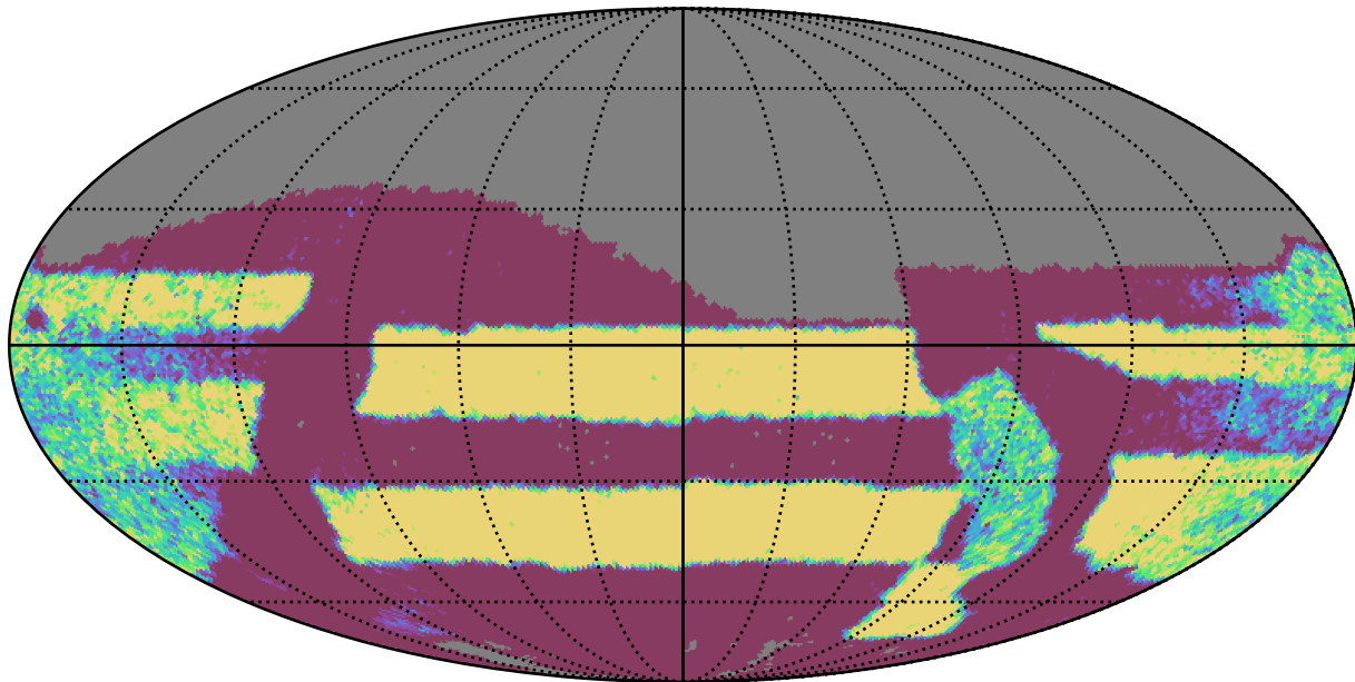
baseline_v2.1_10yrs Yr 3-4 i band: NVisits
