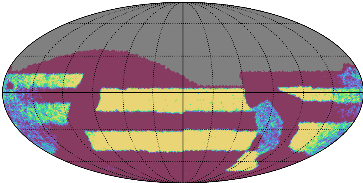
baseline_v2.1_10yrs Yr 3-4 all bands: NVisits
