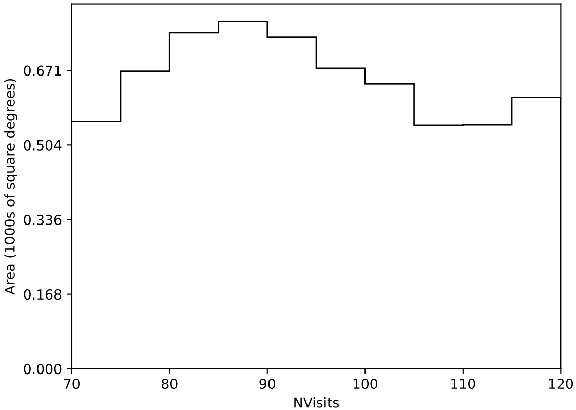
baseline_v2.1_10yrs Yr 3-4 all bands: NVisits
