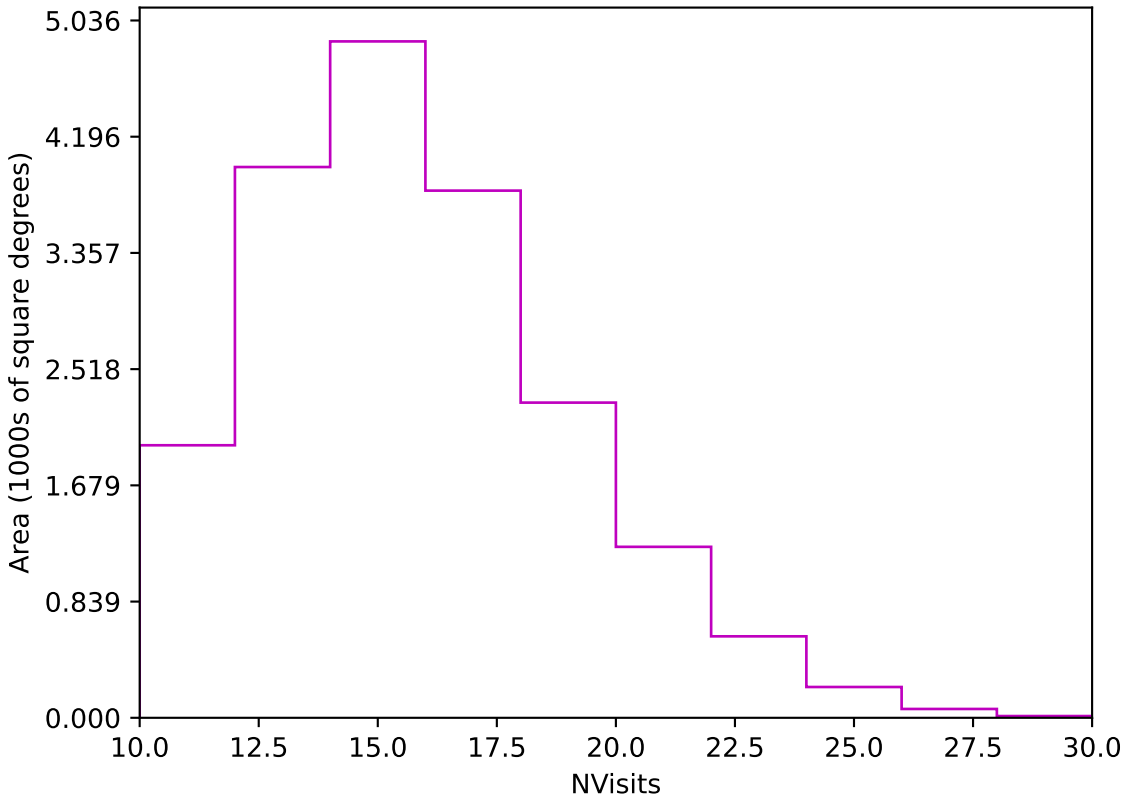
baseline_v2.1_10yrs Yr 1 z band: NVisits
