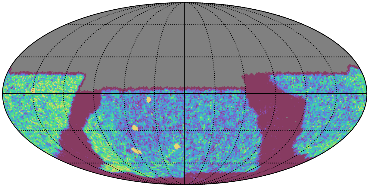
baseline_v2.1_10yrs Yr 1 y band: NVisits
