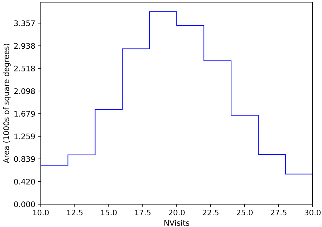
baseline_v2.1_10yrs Yr 1 y band: NVisits
