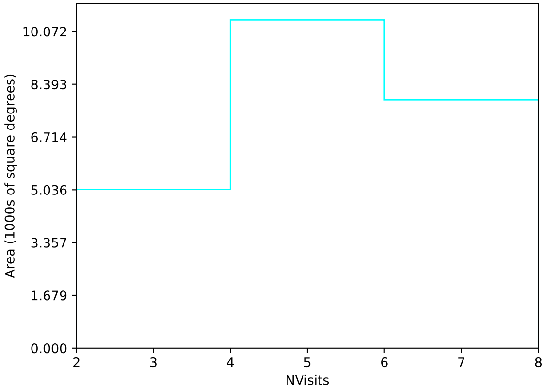
baseline_v2.1_10yrs Yr 1 u band: NVisits
