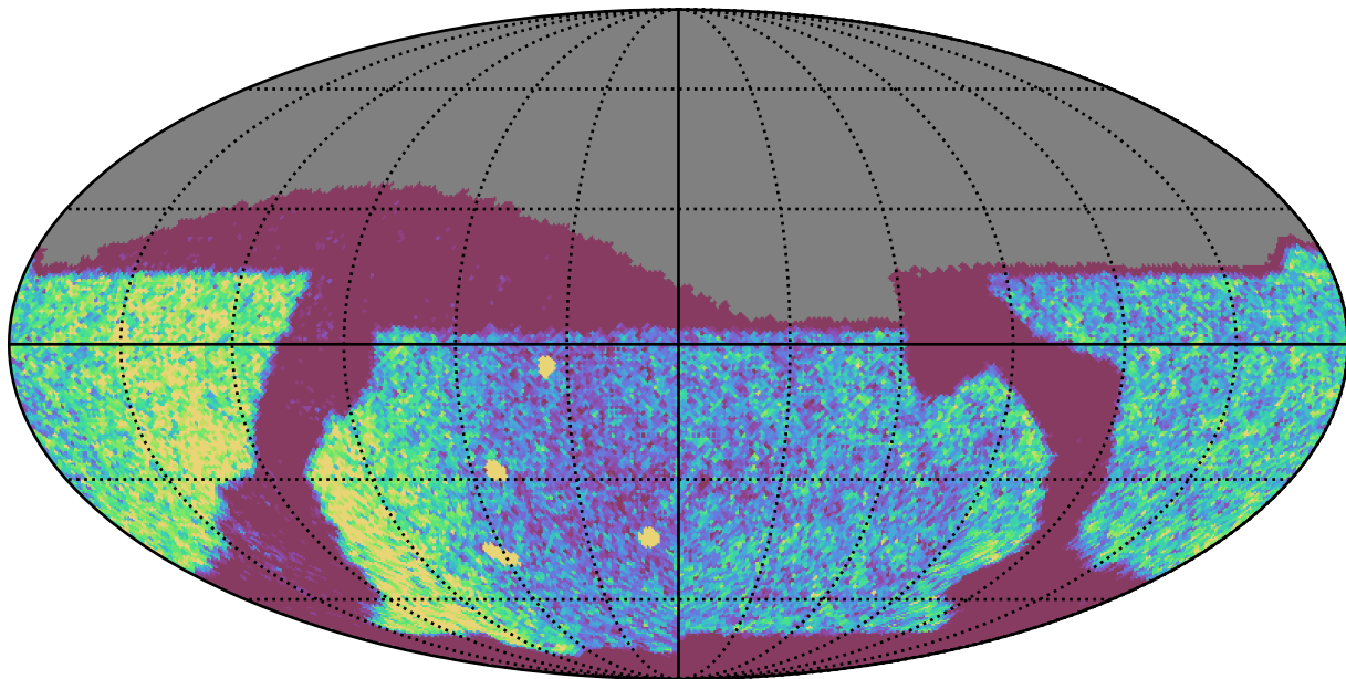
baseline_v2.1_10yrs Yr 1 r band: NVisits
