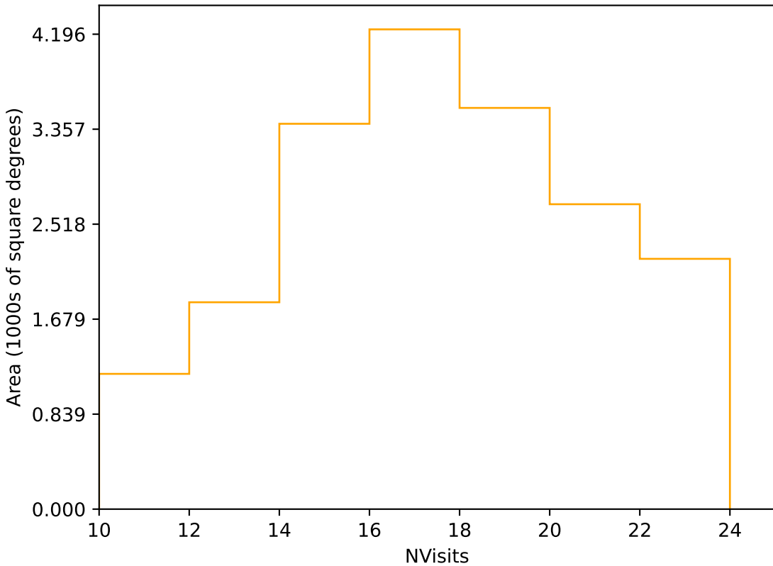
baseline_v2.1_10yrs Yr 1 r band: NVisits
