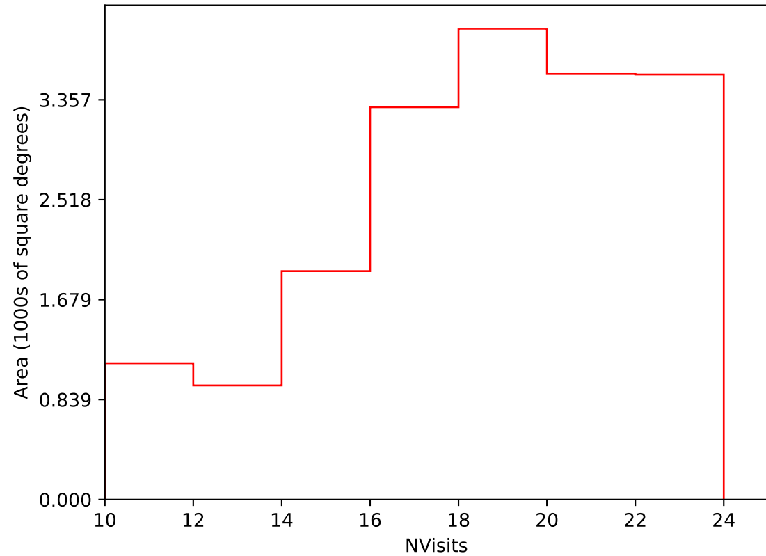
baseline_v2.1_10yrs Yr 1 i band: NVisits
