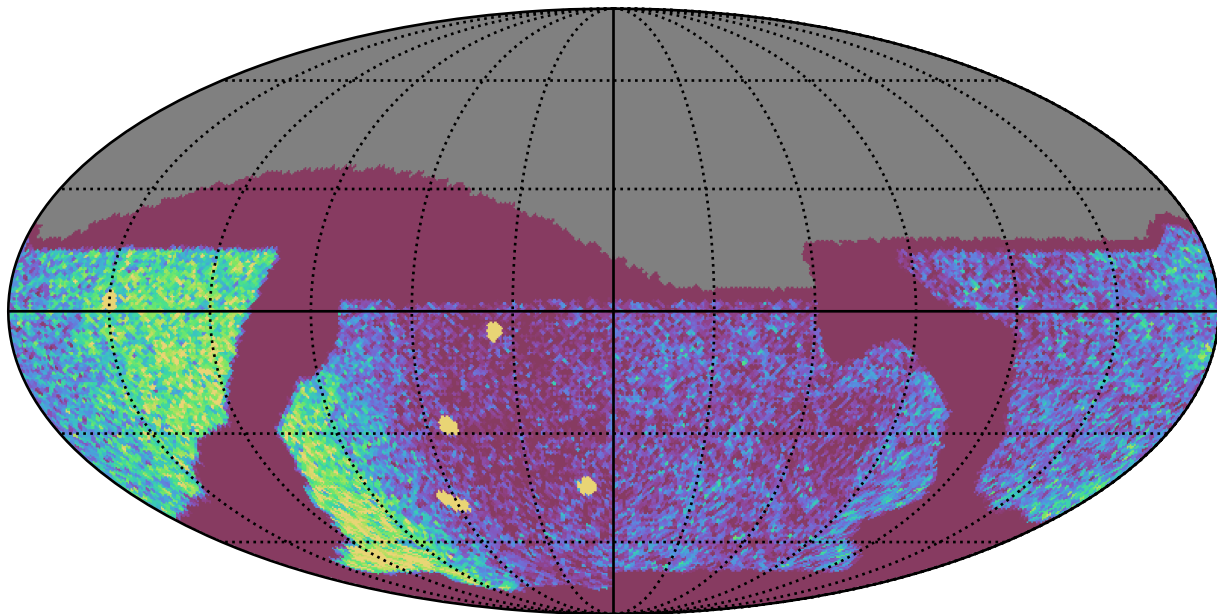
baseline_v2.1_10yrs Yr 1 all bands: NVisits
