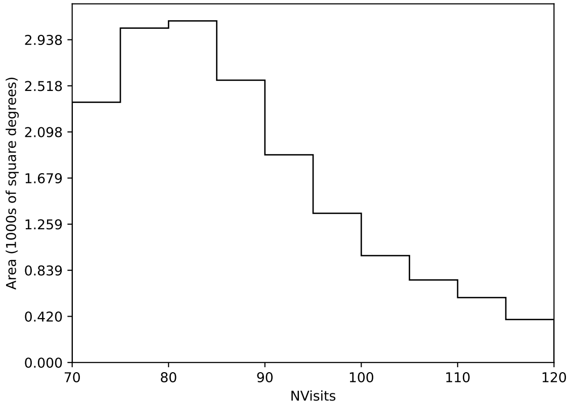
baseline_v2.1_10yrs Yr 1 all bands: NVisits
