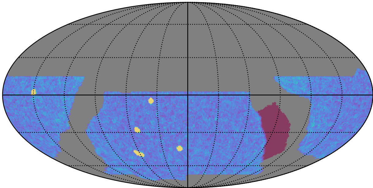
baseline_v2.1_10yrs WFD y band: NVisits
