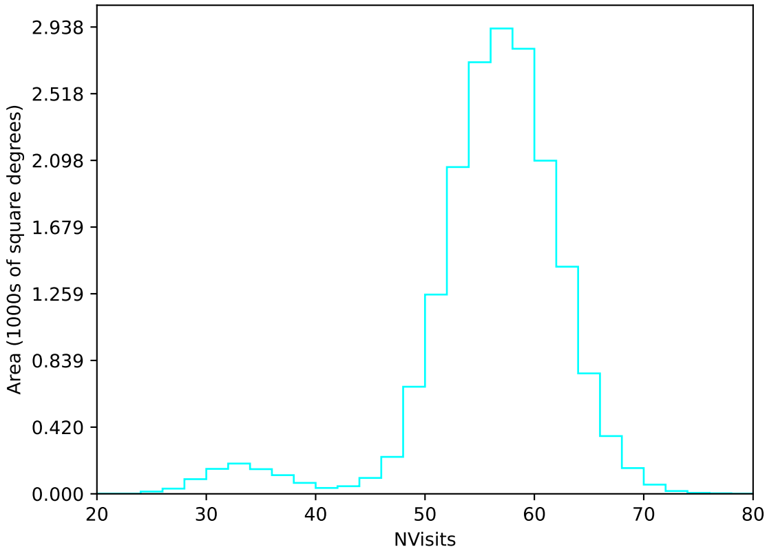
baseline_v2.1_10yrs WFD u band: NVisits
