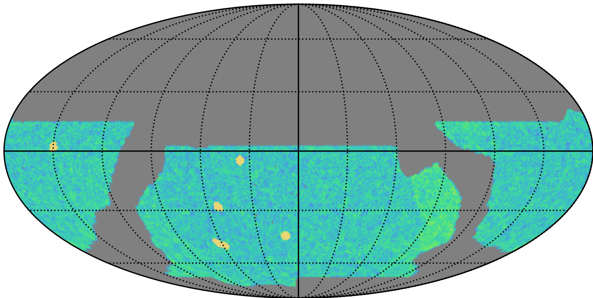
baseline_v2.1_10yrs WFD r band: NVisits
